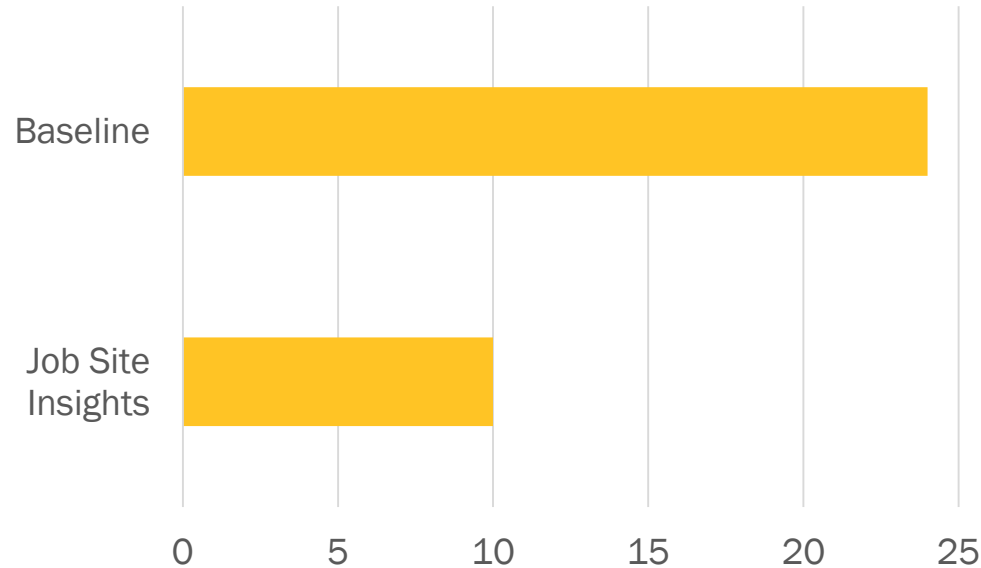
Electric Heater Daily Run Time Hours Comparison
